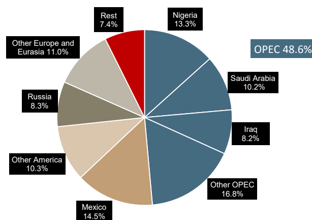
Crude oil import distribution January-November 2016
