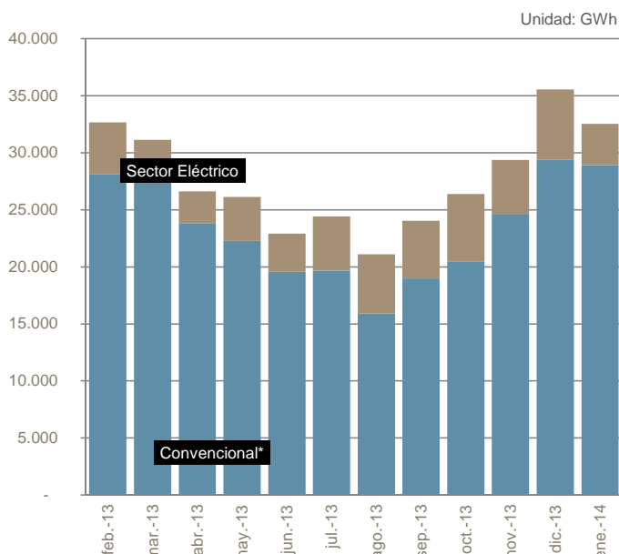
Consumo gas natural feb 2013 - ene 2014
