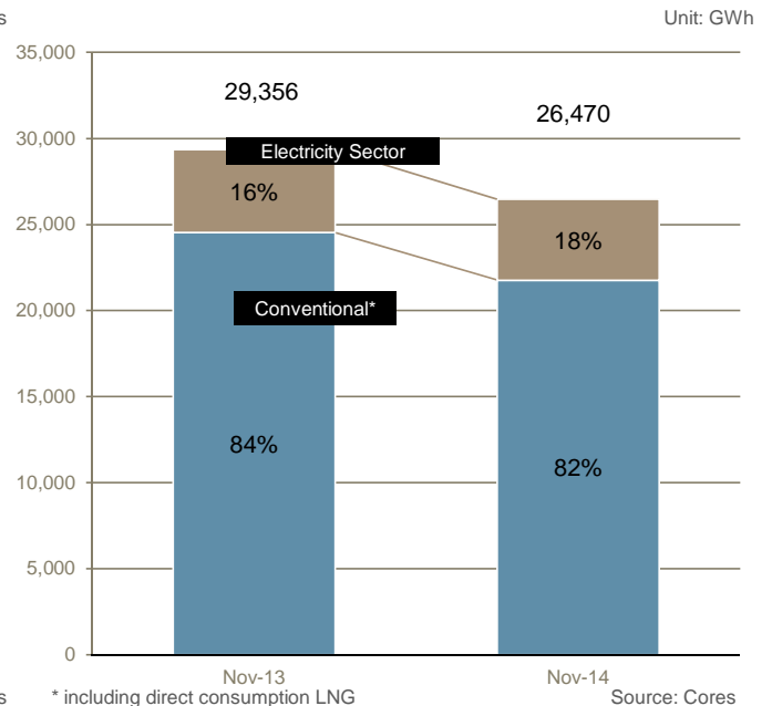
Natural gas consumption Nov. 2013 vs. Nov. 2014
